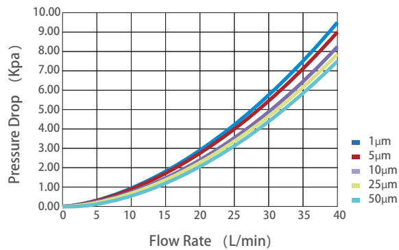
Pressure Drop vs.Flow Rate@20°C
