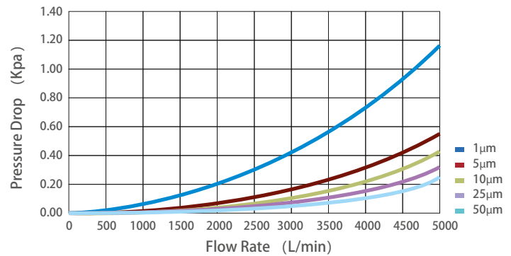
Pressure Drop vs.Flow Rate@20°C
